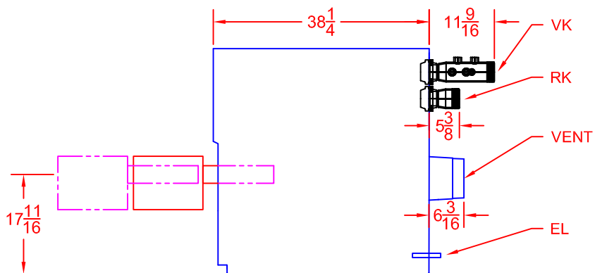
SIDE VIEW
