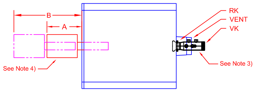
PLAN VIEW
